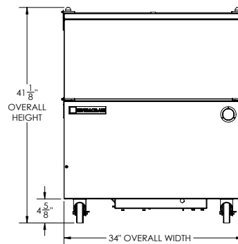
ELEVATION VIEW
